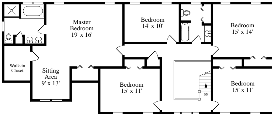
SECOND FLOOR
